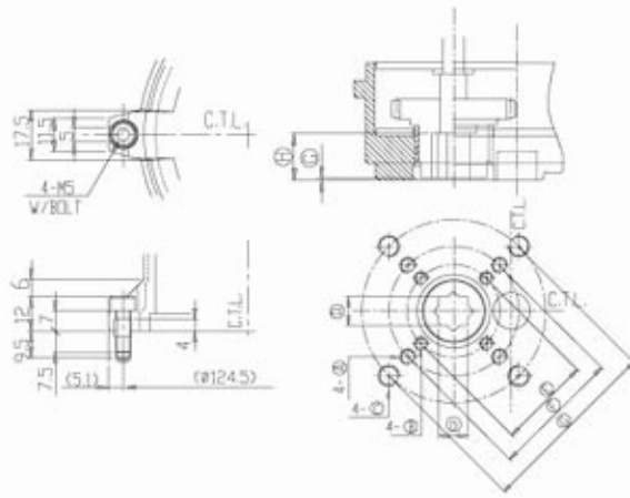
Double square female drive shaft
